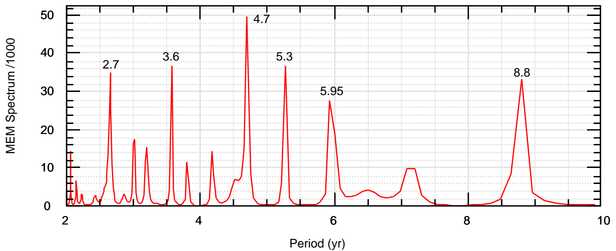
Annual rainfall-South Australia (1900-2018)
