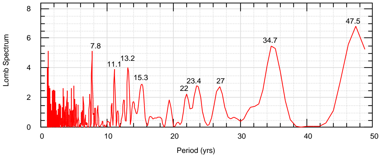
European Temperature Anomaly
