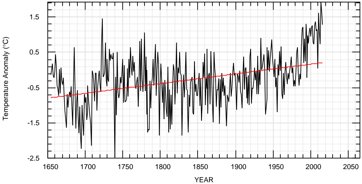
European Temperature Anomaly
