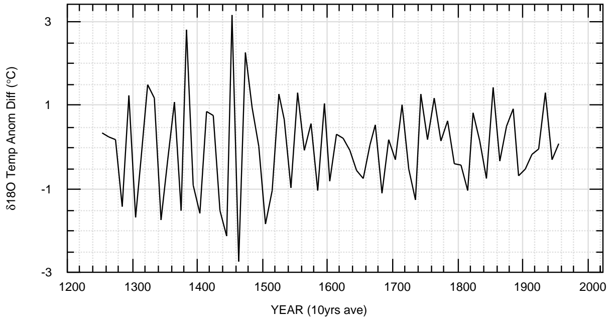
Belukha 2009 Diff \delta^{18}O
