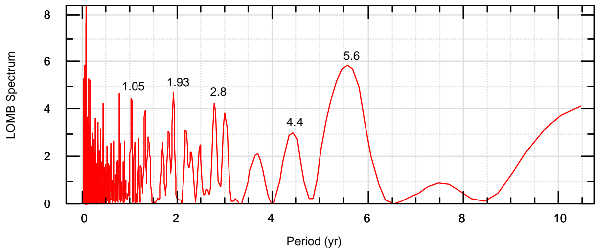
brazil-rain-mo.txt
