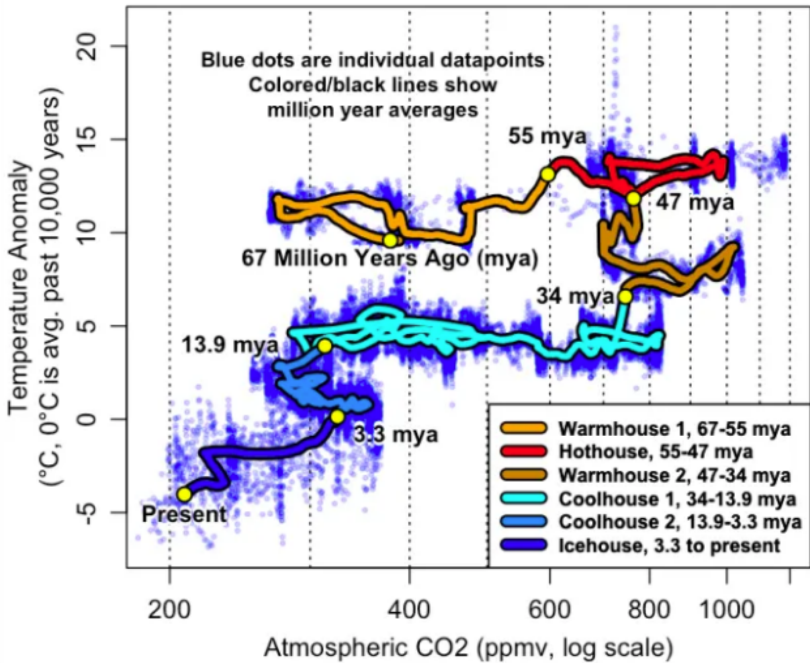
Scatterplot, CENOGRID Temperature vs. Log of Atmospheric CO 2 , 67 million years ago to present
