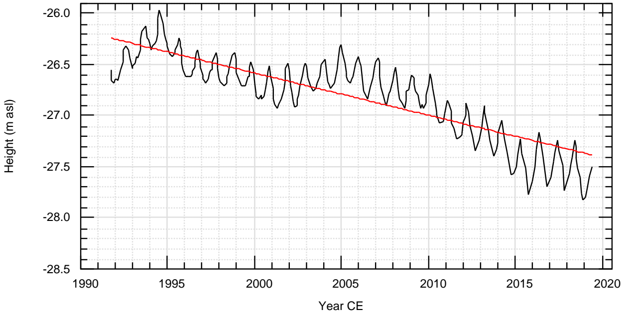
Caspian Level 1992-2019
