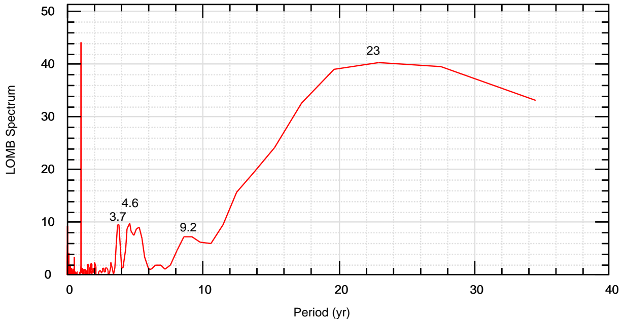
Caspian Level 1992-2019
