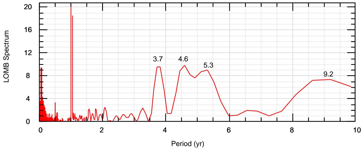
Caspian Level 1992-2019
